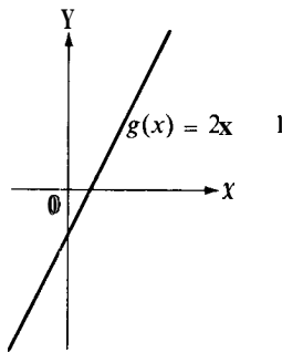
FIGURE 1.9 A linear function g(x) = 2x - 1 .
