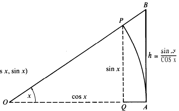
FIGURE 2.9 Geometric proof of the inequalities 0 < \cos x < \frac{\sin x}{x} < \frac{1}{\cos x} .
